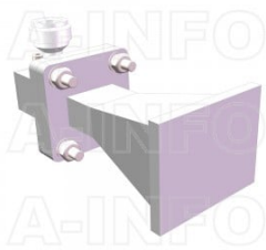
LB-75-10-C-NFSPO Standard Gain Horn Antenna 10-15GHz 10dB Gain N Type Female
